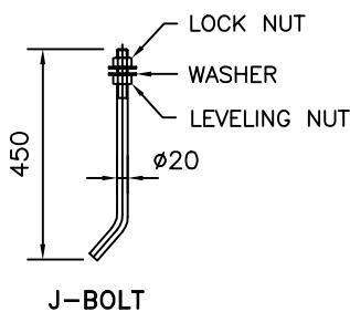
J-BOLT
