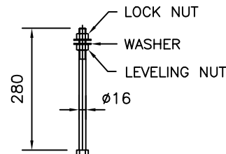
J-BOLT
